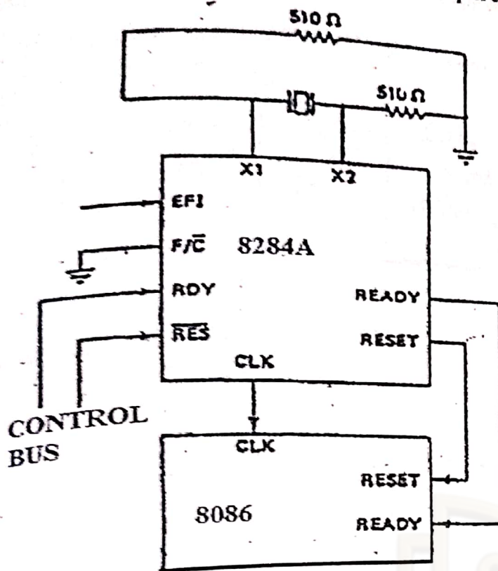
Fig. Connection of 8284A with 8086 microprocessor
