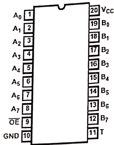
Figure: 8286 Transceiver
