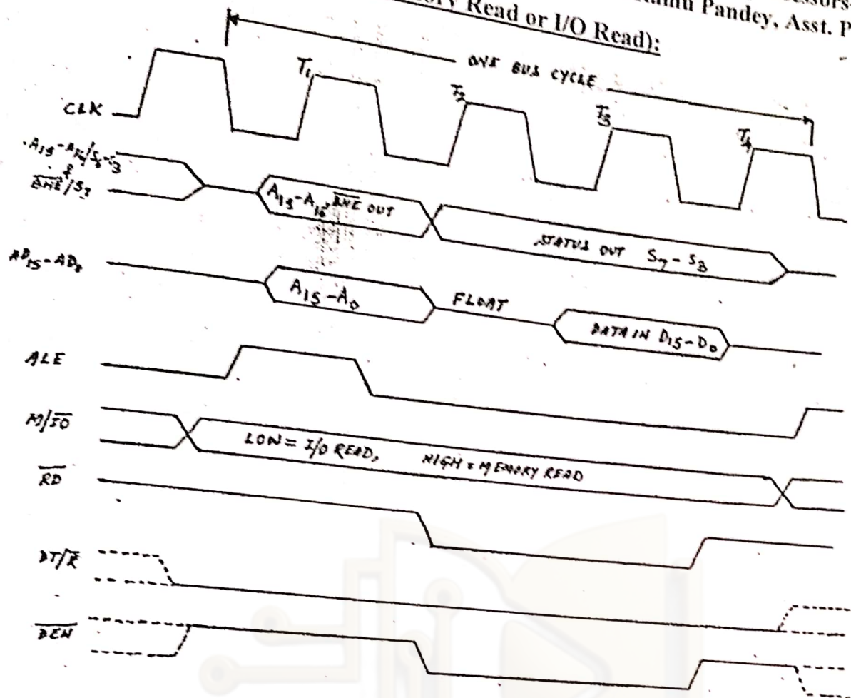
Fig. Bus Cycle For Minimum mode ( I/O Read or Memory Read)
